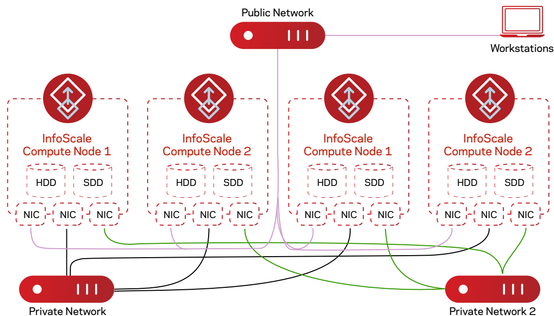
Figure 10. An overview of InfoScale networking between two private networks.
