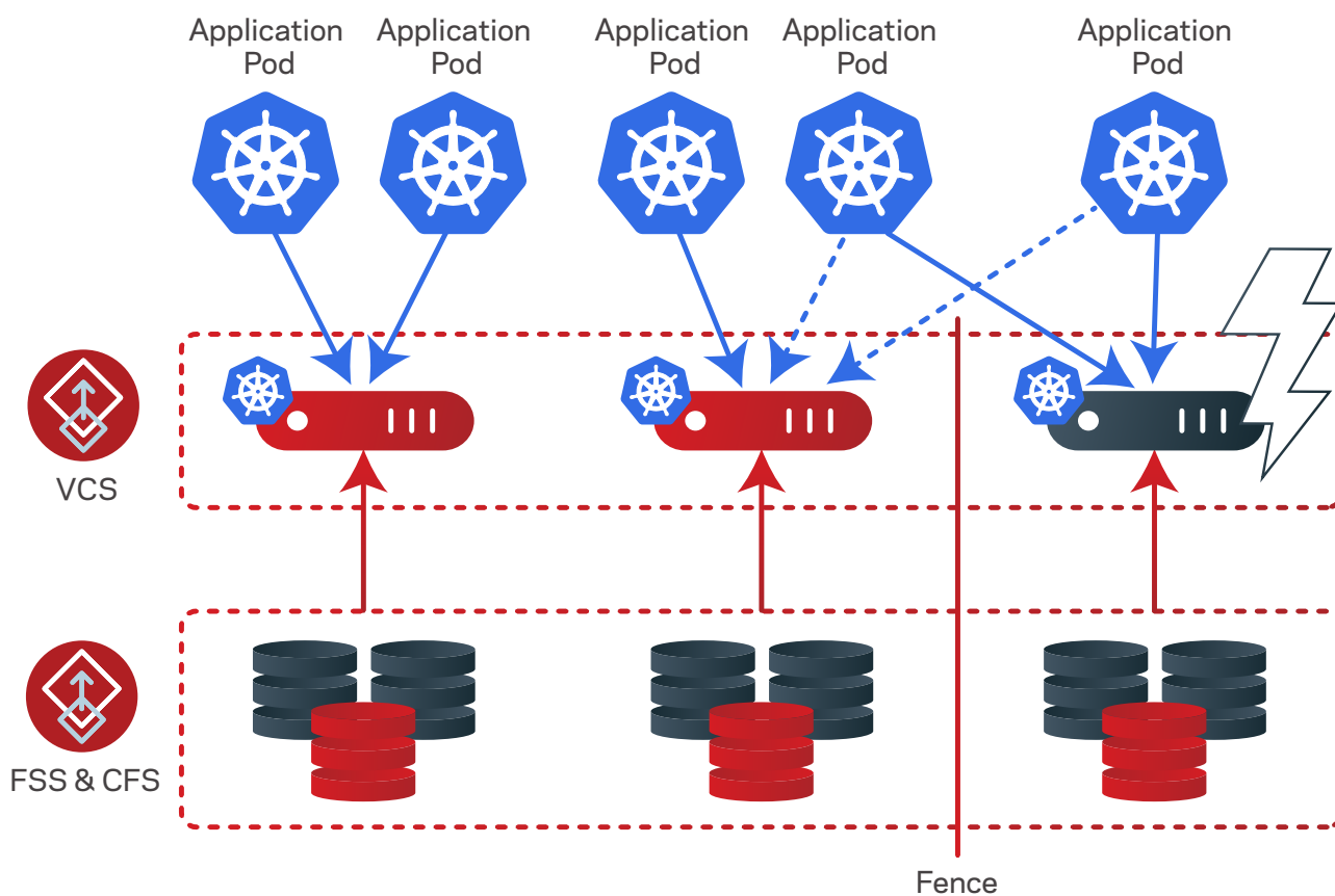
Figure 17. The I/O fencing process in Kubernetes using the InfoScale CSI plug-in.
