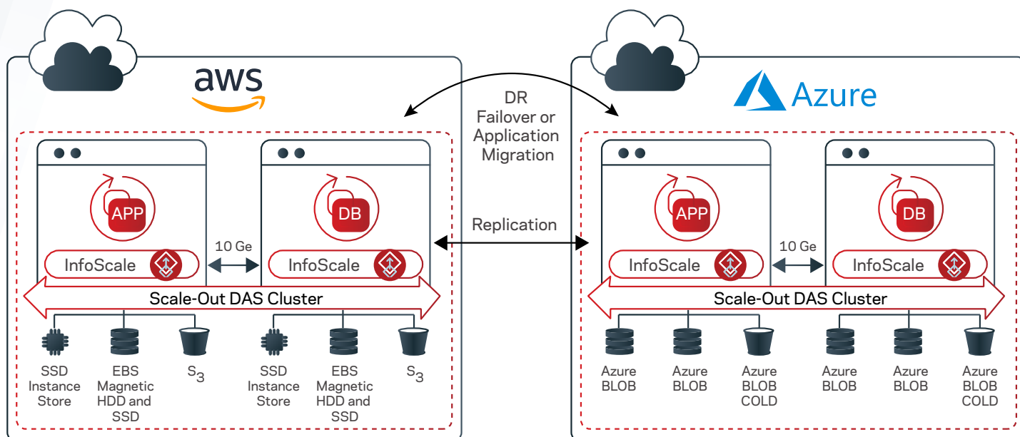
Figure 13. A sample InfoScale public cloud design concept.
