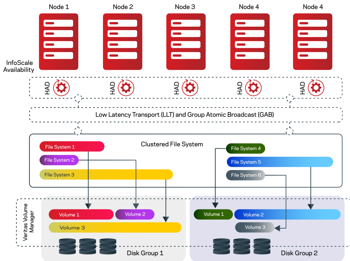
Figure 11. An example of an InfoScale Enterprise solution that includes VCS,CFS and VxVM.
