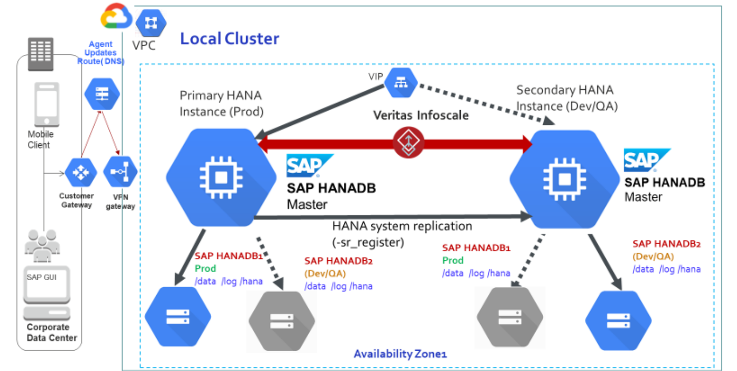
Figure 5. If an SAP HDB instance in production fails, InfoScale will detect the SAP HDB instance failures and non-disruptively fail over the instances between the designated SAP systems
