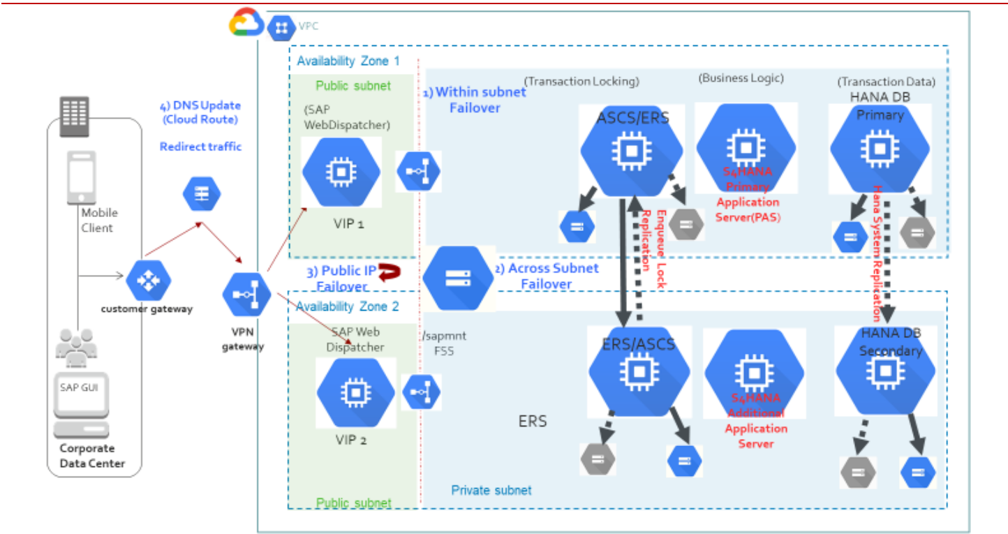
Figure 3. Deployment of an SAP S/4HANA application server with an SAP HANA database on GCP
